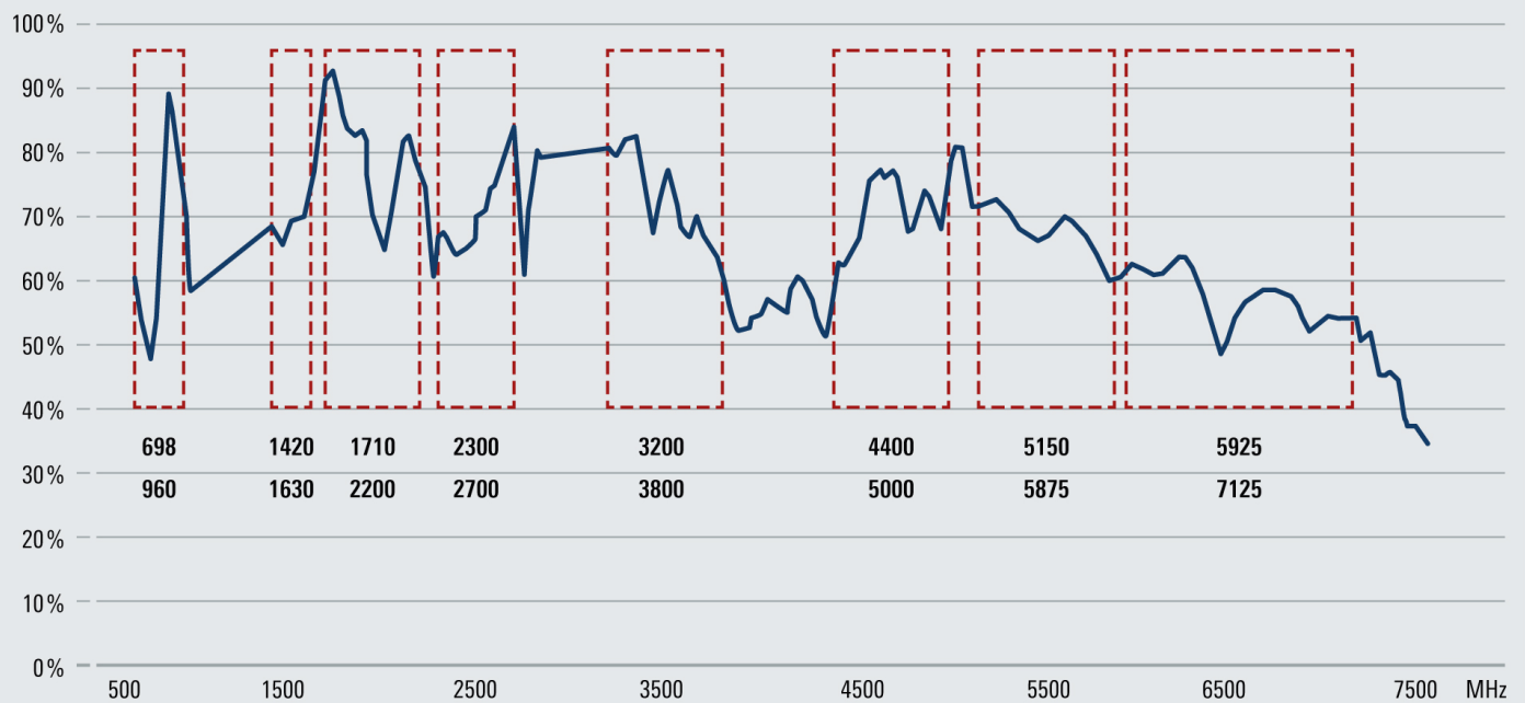
Figure 4-3: Efficiency plot of a 5G NR FR1 MetaSpan antenna
