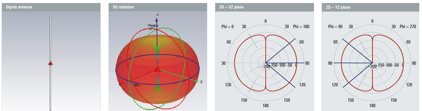
Figure 2-7: Radiation patterns of dipole (omnidirectional) antenna in 3D and 2D
