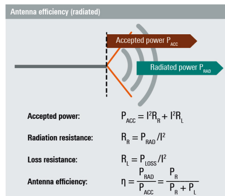
Figure 2-5: Antenna radiation efficiency
