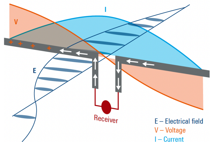
Figure 2-1: Principle of a receiving antenna
