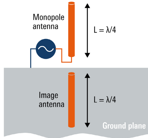
Figure 3-1: Antenna on ground plane
