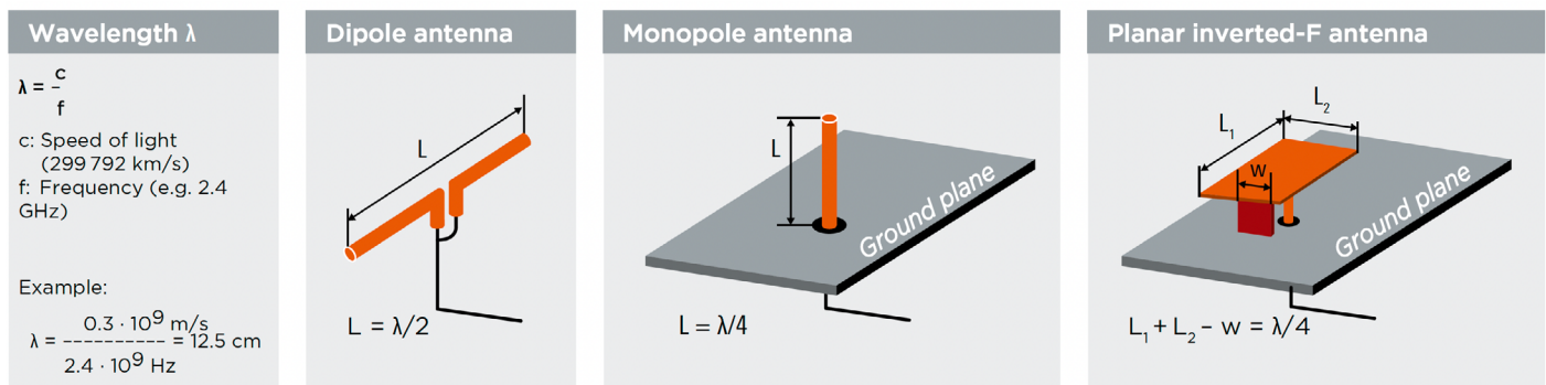
Figure 2-2: Wavelength/dimensions of different types of antennas
