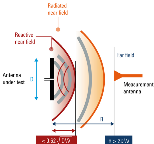
Figure 5-2: Far field condition criteria
