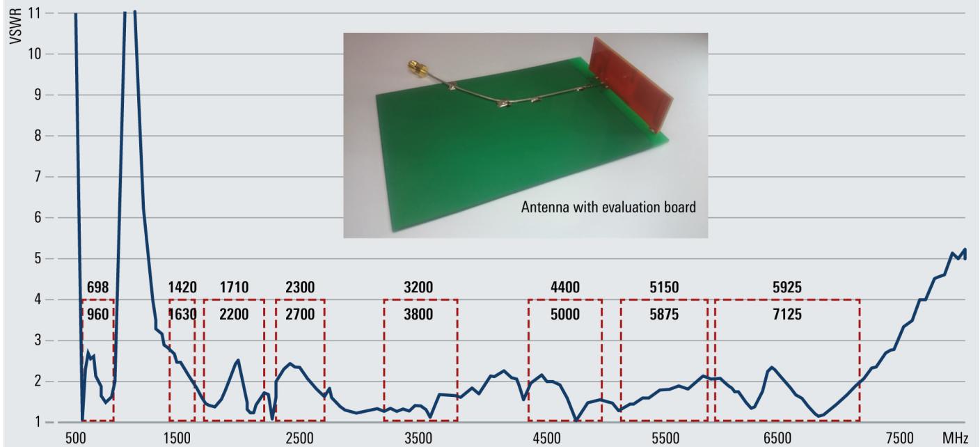
Figure 4-2: VSWR plot of a 5G NR FR1 MetaSpan antenna
