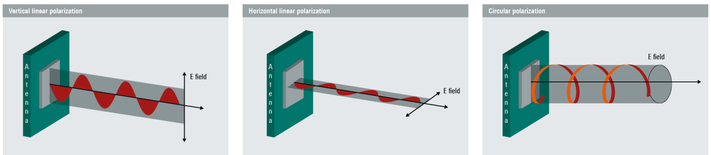
Figure 2-6: Various antenna polarization schemes
