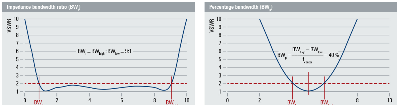
Figure 2-4: Bandwidth parameters defined by VSWR ( \leq 2 )
