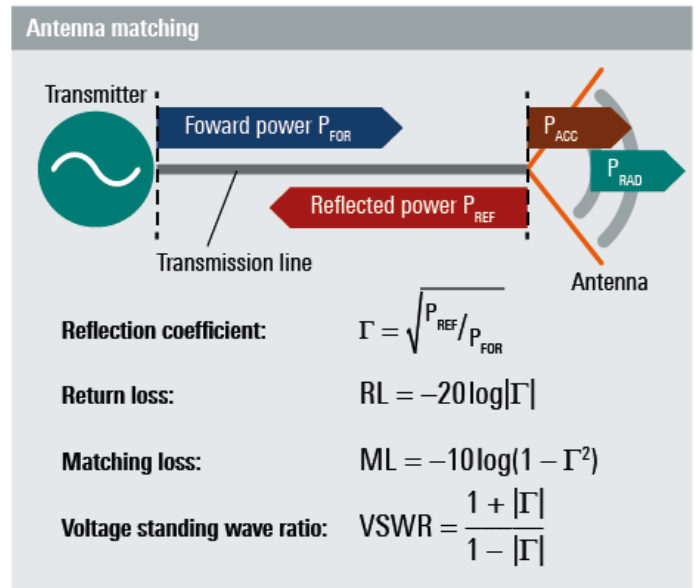
Figure 2-3: Antenna matching parameters
