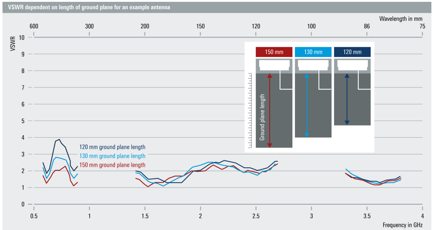
Figure 3-2: VSWR dependent on length of ground plane
